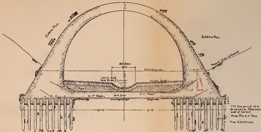
SECTIONAL ELEVATION OF CONDUIT.
